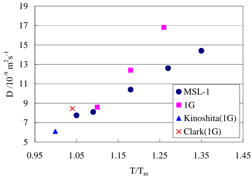
図6. PbSnTe融体の相互拡散係数 MSL-1, 1G: Uchida et al (JASMA, 16, 38, 1999) Kinoshita(1G): Kinoshita and Sugii(J. Crystal Growth, 67,375,1984) Clark(1G): Clark et al. (J. Electrochem. Soc., 130, 164, 1983)
